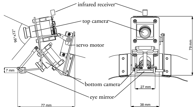
Fig. 2. Schematics of the WearCam, with the two CCD cameras, servo motor and mirror reflecting the eyes of the child.
