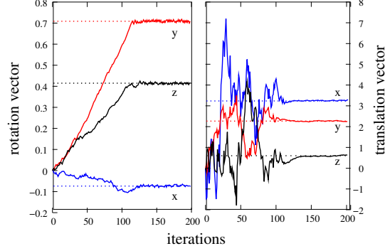
Figure 1: Convergence of the algorithm. The three vector components are indicated by x , y and z . The dotted horizontal lines are the true parameter values of rigid body transformation and the solid lines show the evolution of the estimated values using the learning algorithm.
